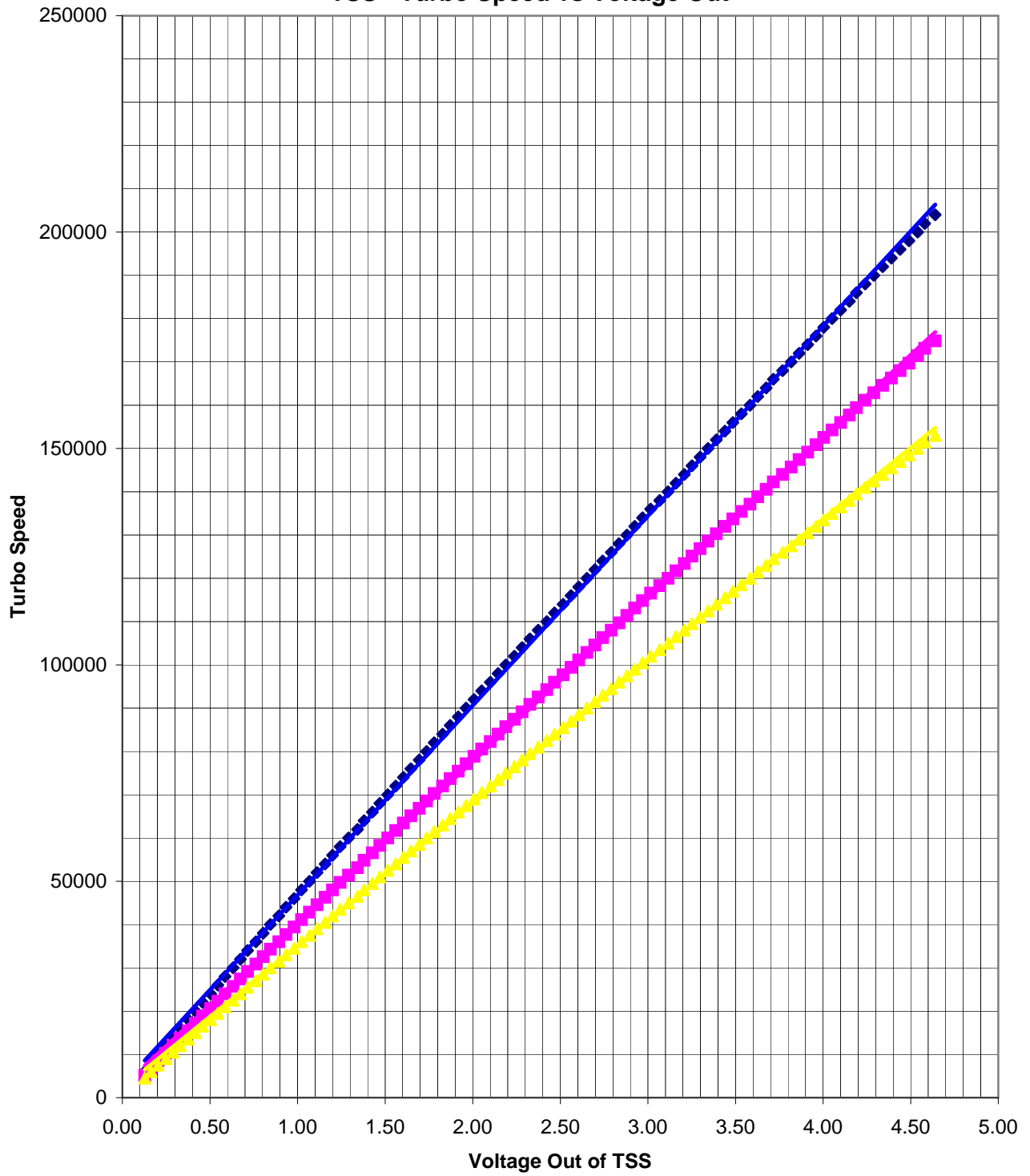
TSS - Turbo Speed vs Voltage Out
